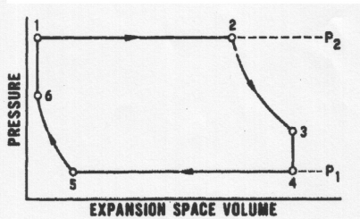
Fig. 2-7. Solvay Refrigeration Cycle
