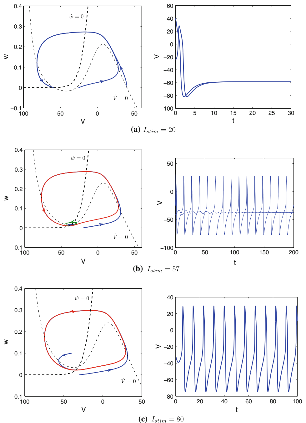
Fig. 3 Examples of phase portraits ( left ) and waveforms ( right ) when \beta_m = 0 . Red and dark green closed curves in phase portraits (b), and (c) denote stable and unstable limit cycles, respectively. Arrows indicate directions of trajectories. Light and heavy dashed curves indicate V - and w -nullclines of model (1) (color figure online)
