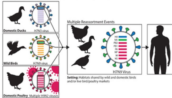
Genetic Evolution of H7N9 Virus in China, 2013
