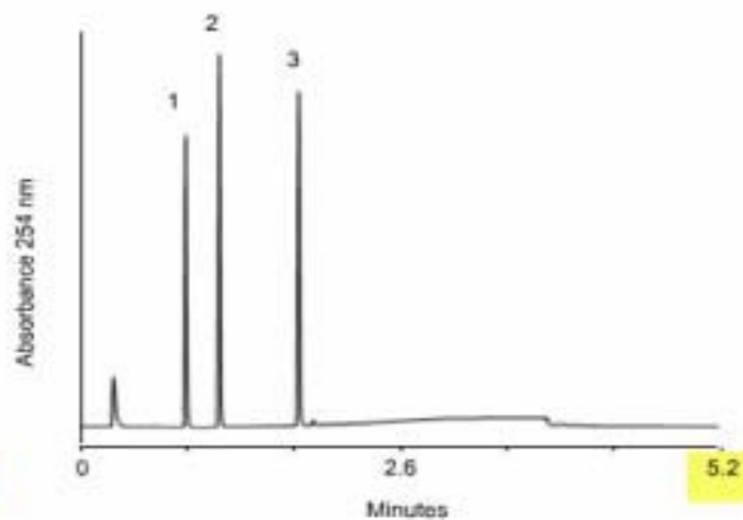
Converted 5.2 minute UPLC™
