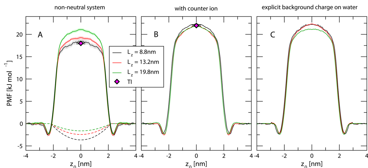
Figure 5. Self-interaction of a test charge (A) PMFs for the non-neutralized systems of different box heights L_z of 8.8 nm (black), 13.2 nm (red), and 19.8 nm (green). PMFs are shown as solid lines with one SD as shaded area. The dashed lines show \delta V(z_0) due to the stabilization of the test particle (charge e/4 ) in the low-dielectric due to its own neutralizing background charge. (B) Respective PMFs with a counterion (charge -e/4 ) in the bulk water, and (C) with an explicit background charge only in the water. Diamond: Free energy difference between hexadecane and water from thermodynamic integration.
