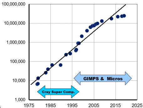
Digits in Largest Known Prime by Year (microcomputer age)
