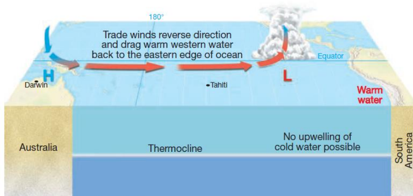
(b) Circulation during El Niño
