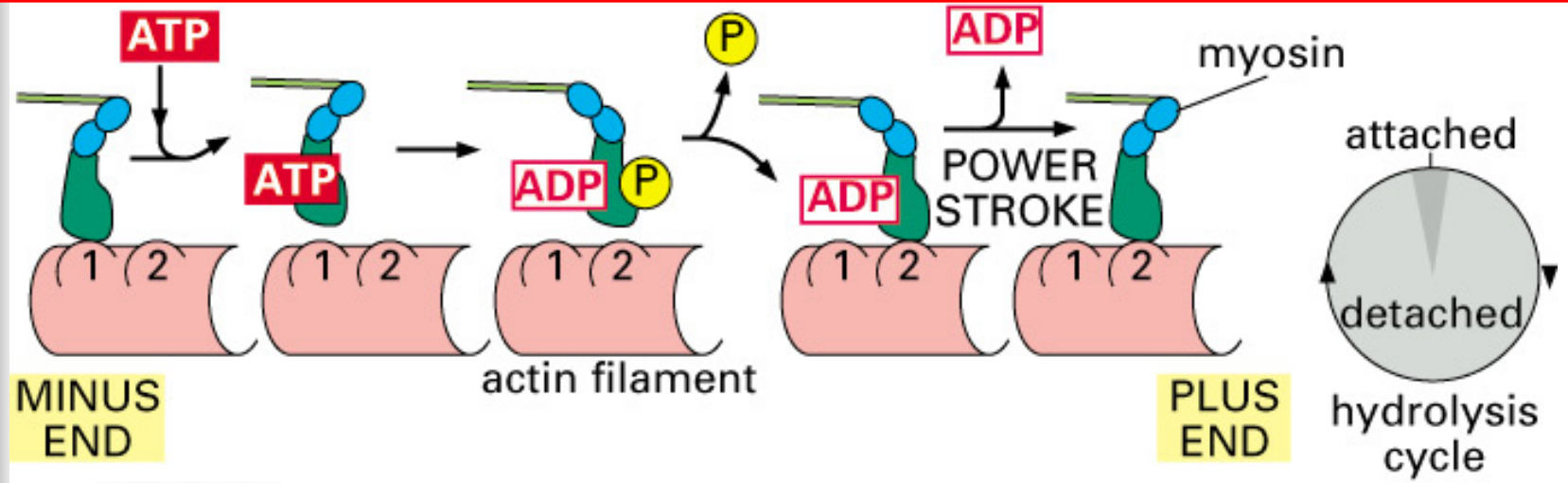
(B) MYOSIN
