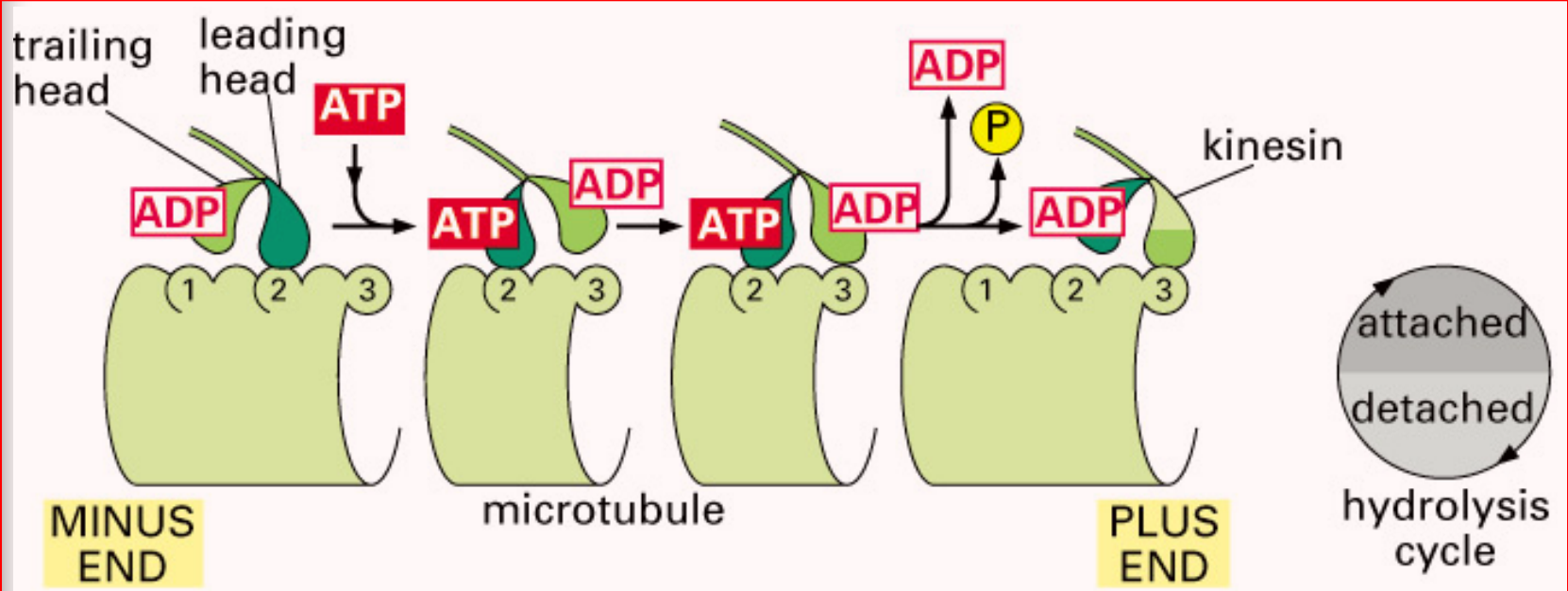
(A) KINESIN
