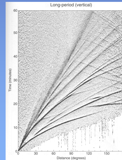
Fig. 4.20. A stack of long-period ( > 10 s), vertical component data from the global network between 1988 to 1994. See Figure 4.23 for a key to the phase names. (From Astiz et al., 1996.)
