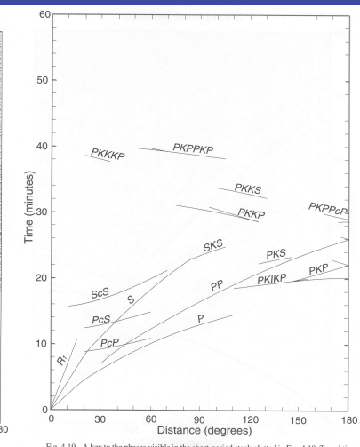
Fig. 4.19. A key to the phases visible in the short-period stack plotted in Fig. 4.18. Travel time curves are calculated using the IASP91 velocity model (Kennett and Engdahl, 1991). (From Astiz et al., 1996.)
