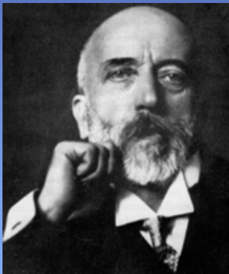
Andrija Mohorovicic (1857-1936)
