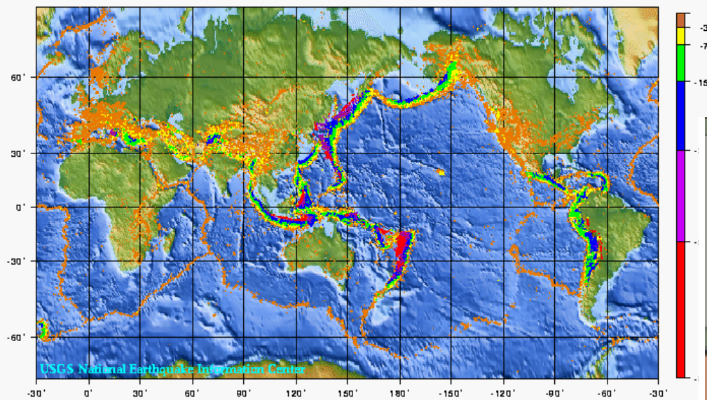
World Seismicity: 1975 - 1995
