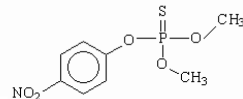
Methyl Parathion
