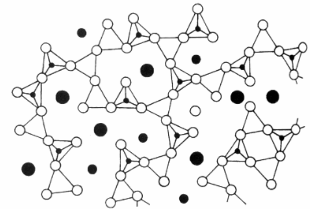
LIQUID \text{CaMgSi}_2\text{O}_6
