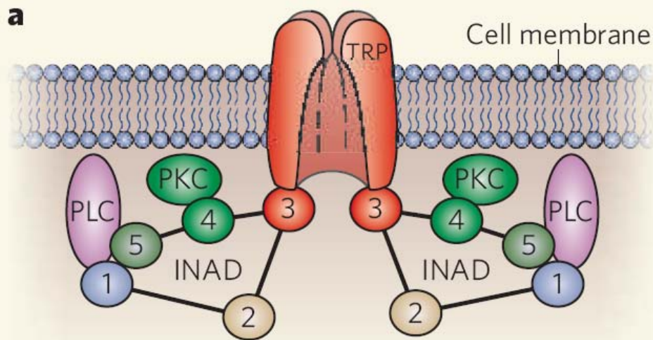
Figure 1 | Phototransduction in Drosophila and the INAD complex. a , The five PDZ domains of INAD (1–5) assemble components of the phototransduction cascade, including PLC, the TRP channel and PKC, into a signalling complex at the cell membrane. b , Mishra et al. 2 report that, in response to light, the PDZ5 domain of INAD undergoes a conformational change. In the dark, PDZ5 is in its canonical, reduced form, in which a groove between an \alpha -helix and a \beta -sheet serves as a ligand-binding site. After stimulation with light, the PDZ5 domain undergoes a conformational change to an oxidized state, whereby the formation of a disulphide bond between two cysteine residues results in the unravelling of the \alpha -helix and the distortion of the ligand-binding groove. Following this conformational switch, the ligand (arrowed) — putatively part of the PLC enzyme — can no longer bind. (Adapted from ref. 2.)
