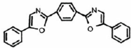
POPOP
