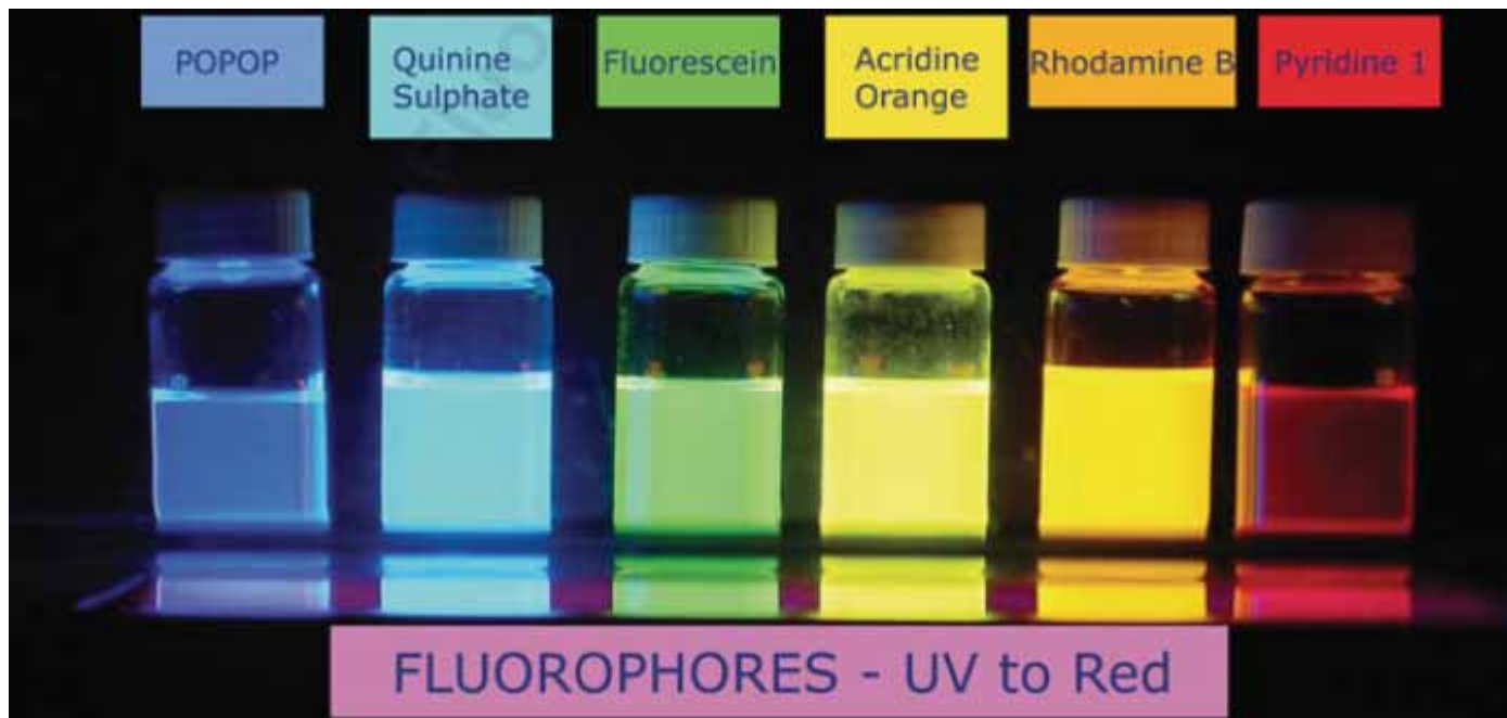
Quinine
