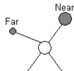
Out-of-plane twisting
