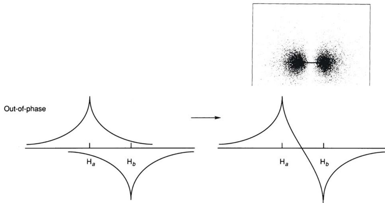
Destructive interference of the waves from two hydrogen 1s orbitals on adjacent atoms (the 'out-of-phase' combination).
