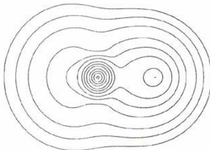
BeH
