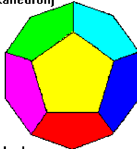
Dodecahedron
