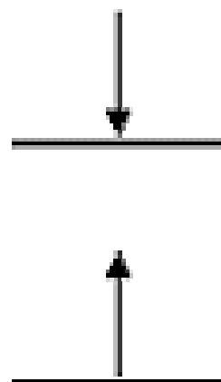
excited singlet state
