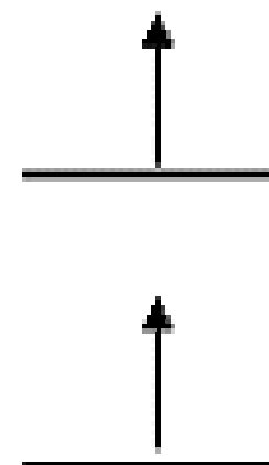
excited triplet state
