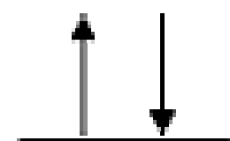
ground singlet state
