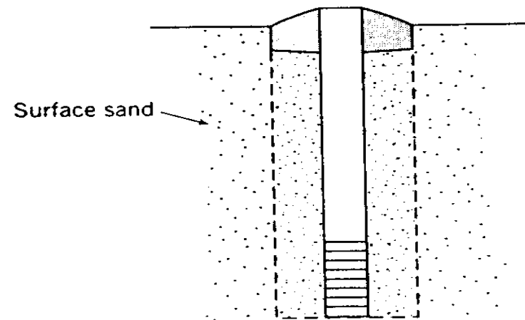
(c) Piezometer Installed in Caving Materials
