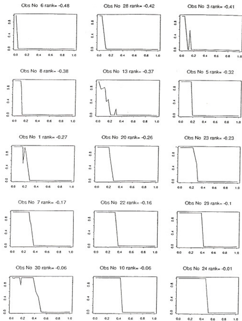
Figure 2.1. Regression rank scores for tobacco data.
