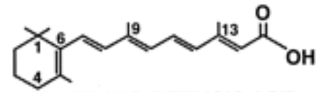
ALL-TRANS-RETINOIC ACID
