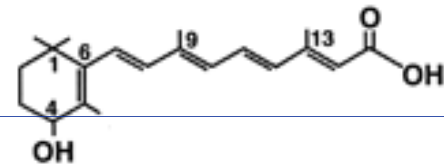
ALL-TRANS-4-HYDROXYRETINOIC ACID
