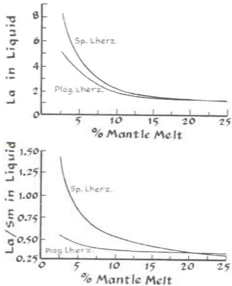
Figure 7-28 (a) Calculated concentrations of La in liquids produced by progressive batch melting of spinel lherzolite and plagioclase lherzolite of the same bulk chemical compositions. (b) La-Sm ratio for the same melts as in (a) La, the lightest of the REE, is not shown in the diagrams of Figure 7-27 but would fall to the left of Ce on the horizontal scale. (After J. F. Allan, R. Batiza, and P. Lonsdale, 1987, Seamounts, Islands, and Atolls , Geoph. Mono. 43, Amer. Geoph. Un., 255-282.)
