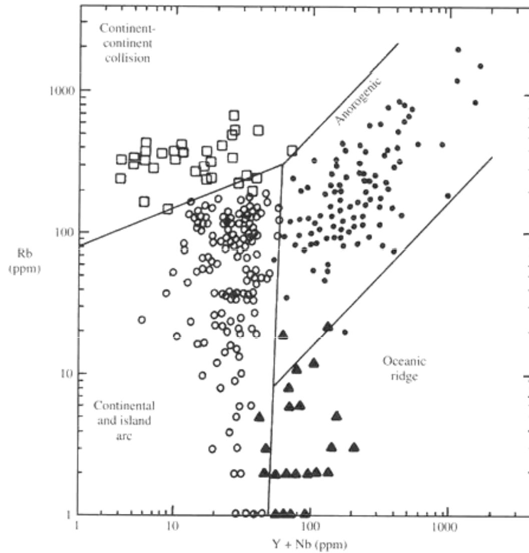
Tectonic discrimination diagram for granitic rocks based on concentrations of Rb versus Y + Nb. Symbols show modern rock suites used to subdivide the diagram. Arc granites broadly correspond to I-type and collision granites to S-type. (Redrawn from Pearce et al., 1984.)
