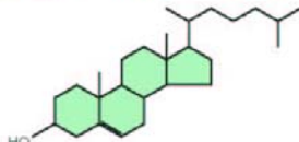
cholesterol —found in many membranes
