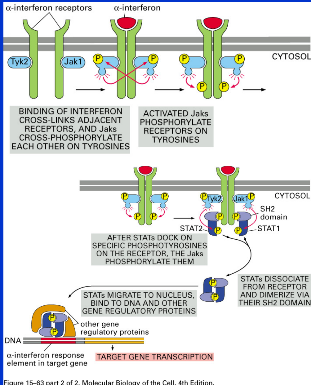
Figure 15-63 part 2 of 2. Molecular Biology of the Cell, 4th Edition.
