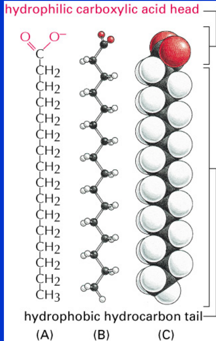
Figure 2-21. Molecular Biology of the Cell, 4th Edition.
