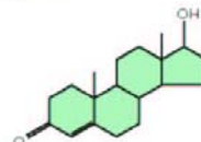
testosterone —male steroid hormone
