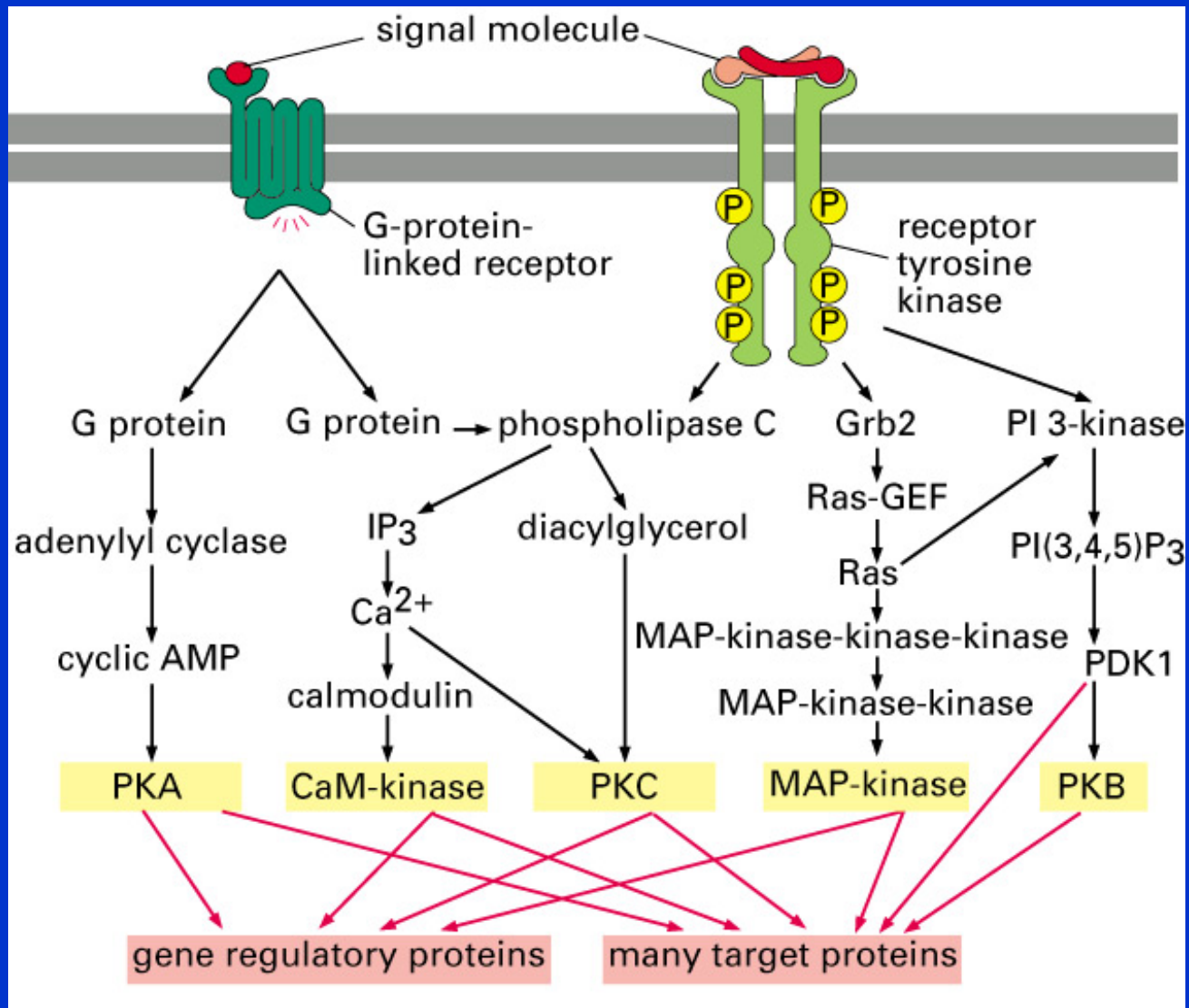
Figure 15-61. Molecular Biology of the Cell, 4th Edition.
