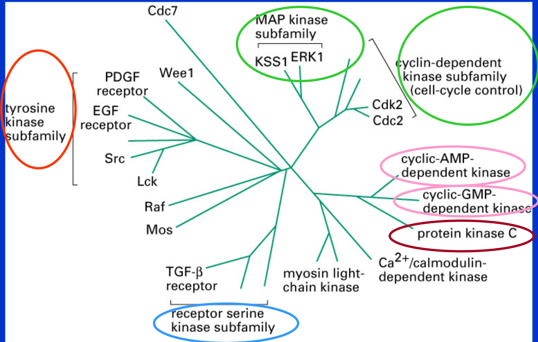
Figure 2-65. Molecular Biology of the Cell, 4th Edition
