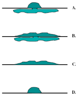
Figure 5. Different morphologies of the colony under different growth conditions quantified by the agar concentration (ac). (a) Diffuse submerging with well-packed non-swarmer colony on surface; very soft surface, ac < 0.4\% . (b) Diffuse submerging with swarmer colony on surface; soft surface, 0.4\% < ac < 0.6\% . (c) Swarmer colony on surface only; intermediate surface hardness, 0.6\% < ac < 1.2\% . (d) Well-packed non-swarmer colony on surface; hard surface, 1.2\% < ac .
