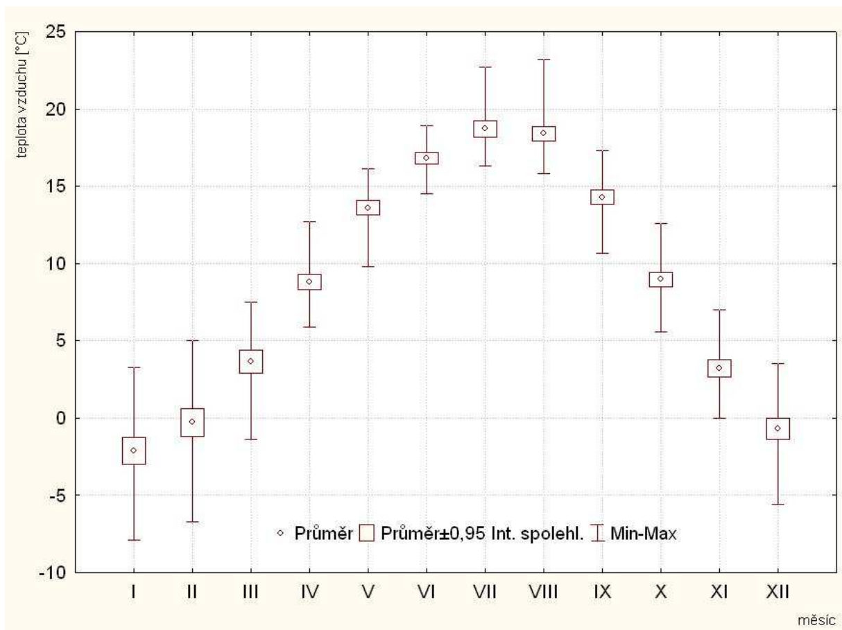
Obr. 5 Box plot
