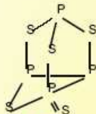
\alpha - P_4S_5
