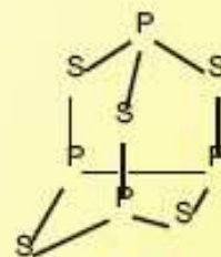
\beta - P_4S_5
