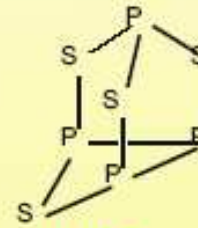
\beta - P_4S_4
