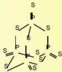
P_4S_{10}
