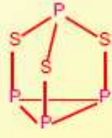
P_4S_3
