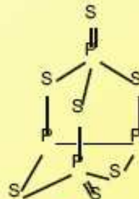
P_4S_7
