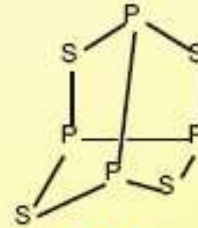
\alpha - P_4S_4
