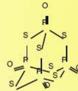
P_4O_4S_6
