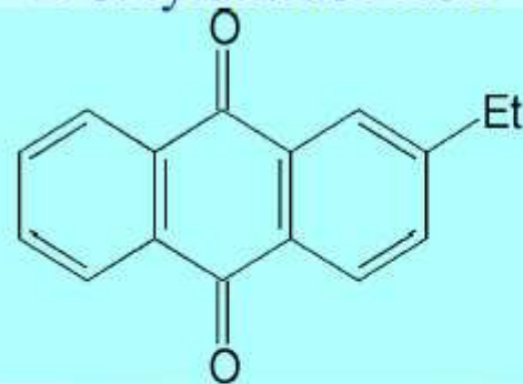
2-ethylantrachinon
