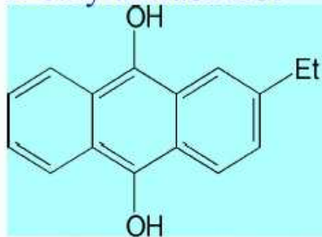
2-ethylantrachinol
