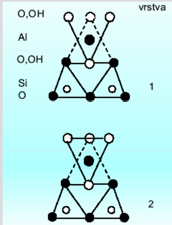
kaolinit \text{Al}_2(\text{OH})_4\text{Si}_2\text{O}_5
