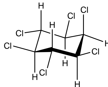
delta-HCH
