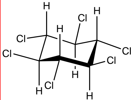
beta-HCH
