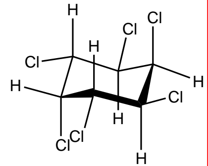
epsilon-HCH
