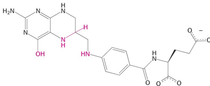
Tetrahydrofolate
