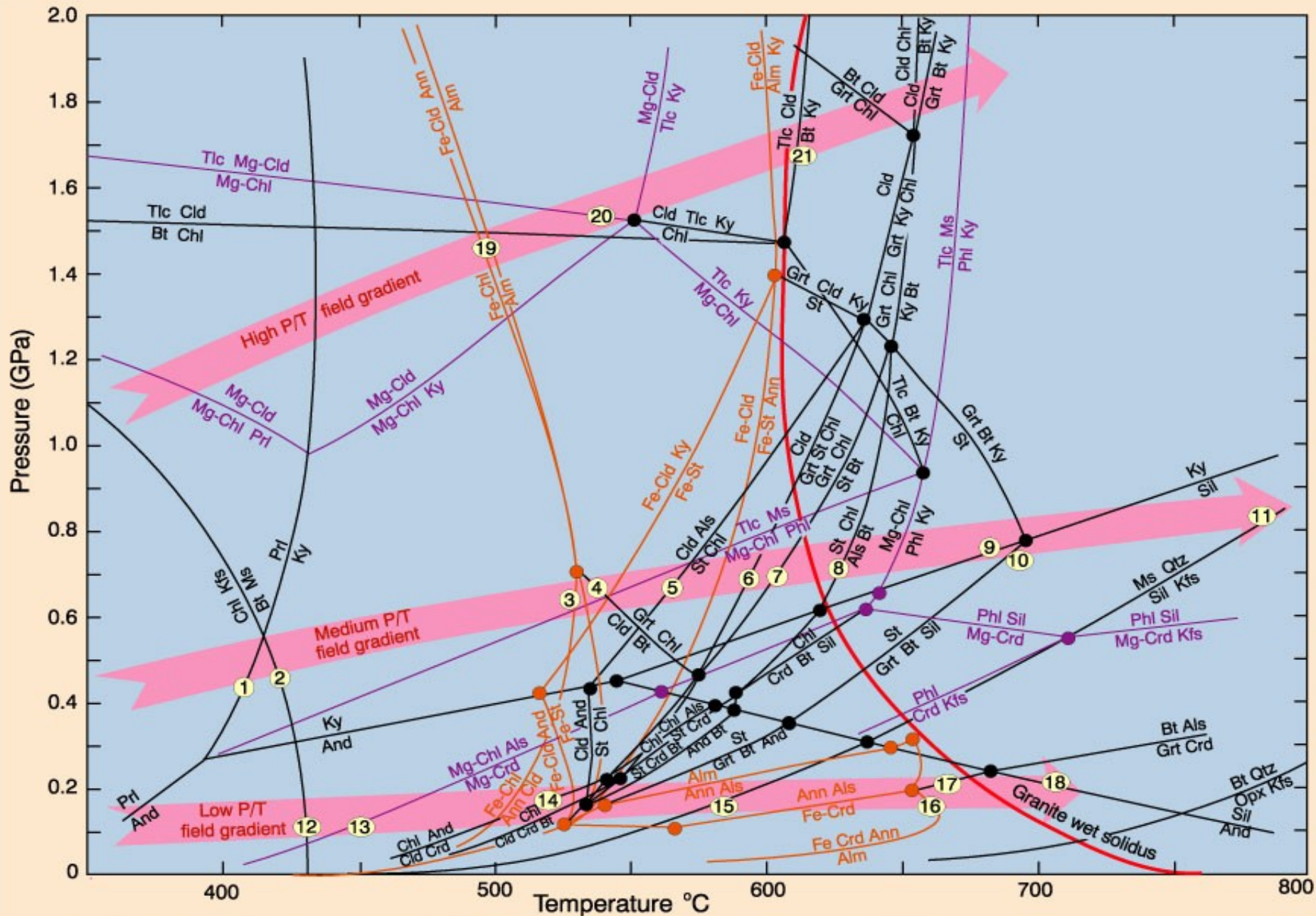
Figure 28-2. Petrogenetic grid for the system KFMASH at P_{H_2O} = P_{total} . Orange curves represent the system KFLASH and purple curves represent the system KMASH. Reactions are not balanced, and commonly leave out quartz, muscovite, and water, which are considered to be present in excess. Typical high, medium, and low P/T metamorphic field gradients are represented by broad pink arrows. After Spear and Cheney (1989), and Spear (1999).
