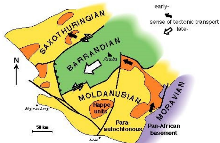
Tectonic evolution of the Bohemian Massif and the juxtaposition of the Barrandian & Moldanubian blocks
