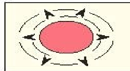
Ballooning
