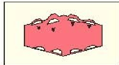
Stopping
