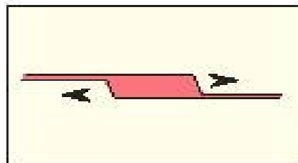
Transcurrent to transpressive
