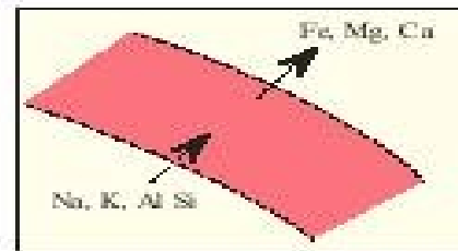
Granitization
