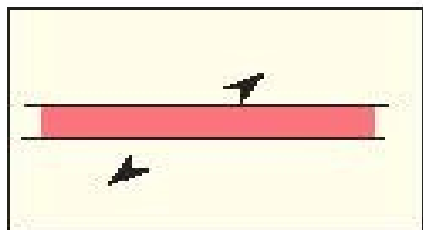
Transensional
