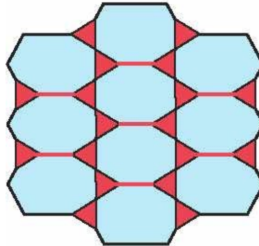
Permeable
