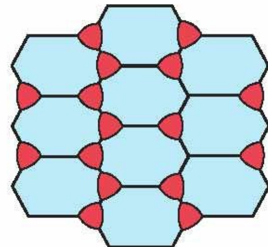
Impermeable
