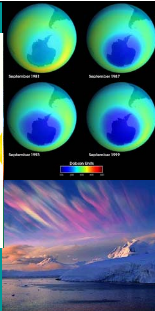
Ozone depletion facilitated by the polar vortex
