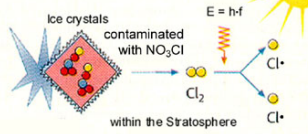
Ozone depletion facilitated by the polar vortex
