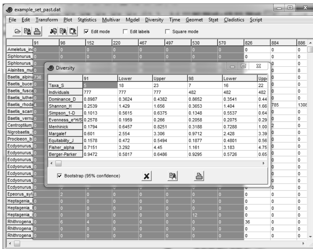
Obr. 10.1 Software PAST
