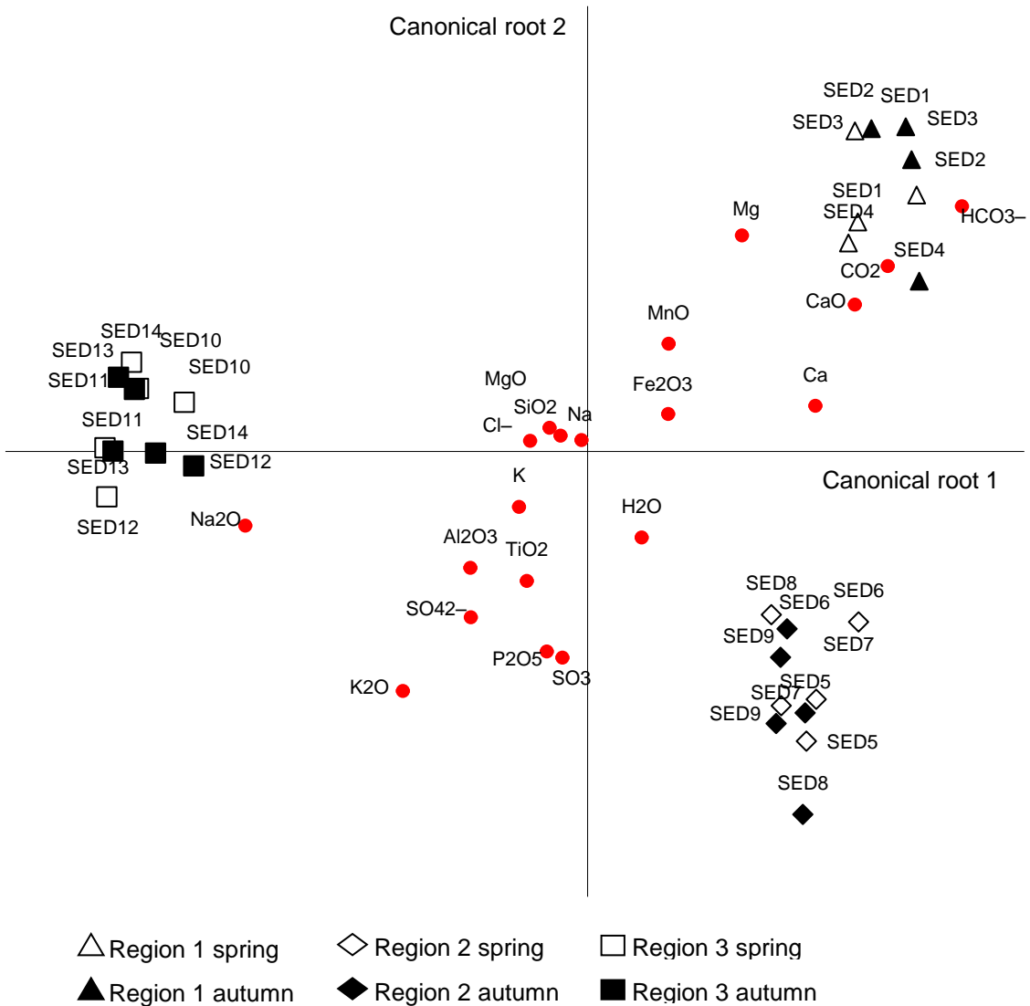
Figure 4. Discrimination plot of hydrogeological regions based on sediment and water geochemistry
