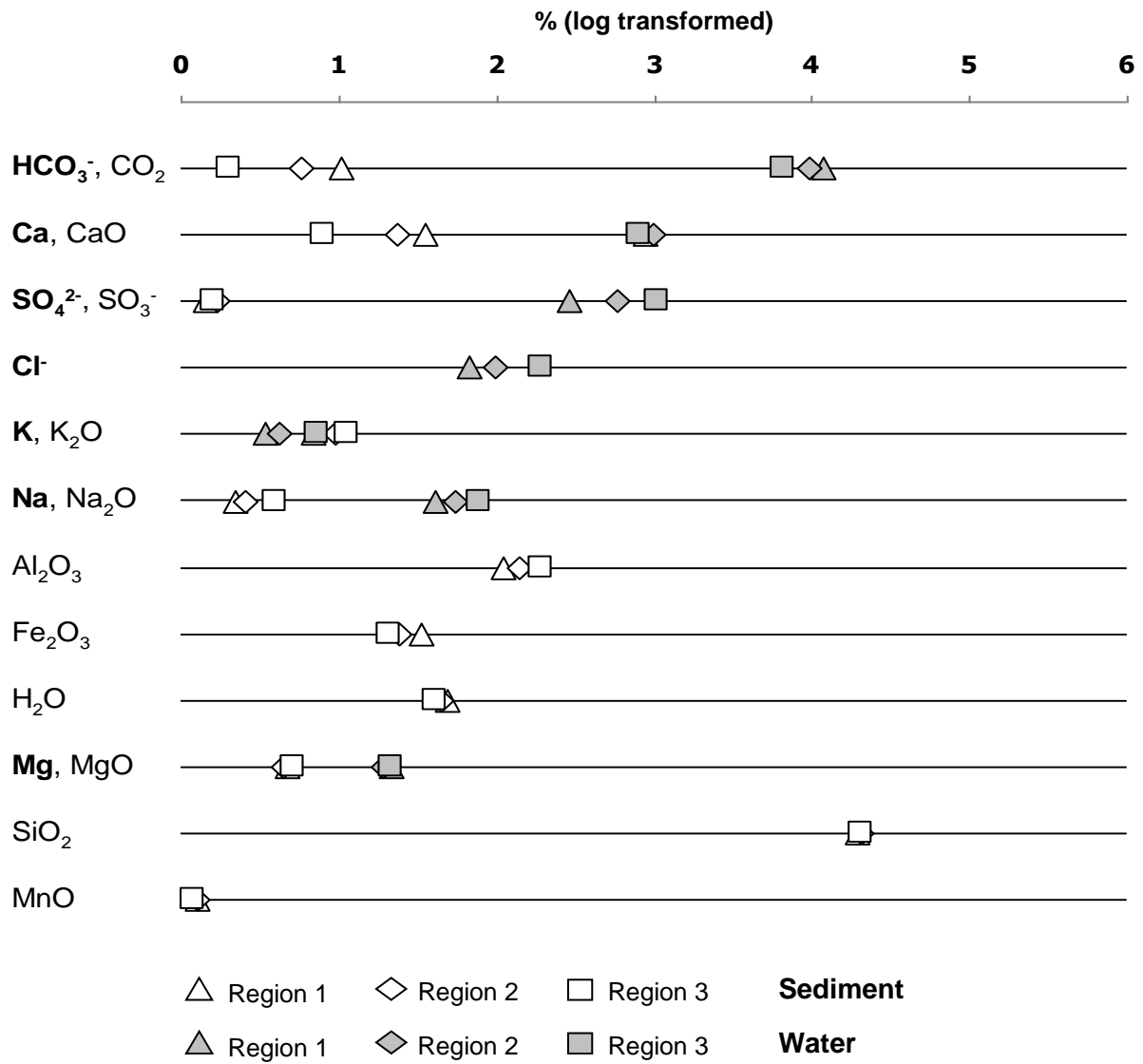
Figure 2. Differences in sediment characteristics among hydrogeological regions. Geochemical characteristics are ordered according to difference among regions (water characteristics are given in bold).
