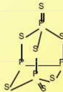
P_4S_7
