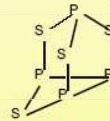
\beta - P_4S_4
