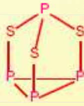
P_4S_3
