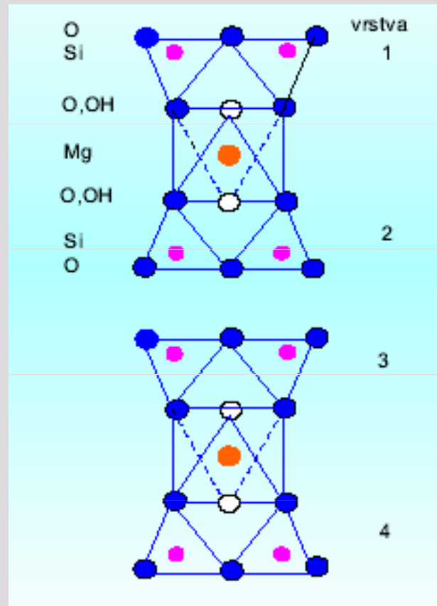
mastek \text{Mg}_3(\text{OH})_2(\text{Si}_2\text{O}_5)_2
