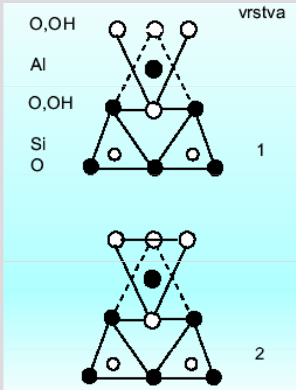
kaolinit \text{Al}_2(\text{OH})_4\text{Si}_2\text{O}_5
