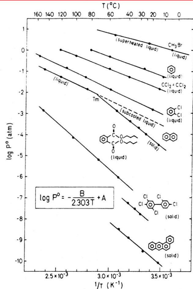
Figure 4.3 Temperature dependence of vapor pressure for some representative compounds.
