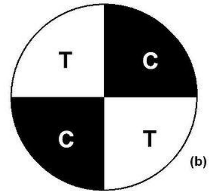
Schematic diagram showing the direction of initial movement of particles around the focus (F) of an earthquake on a W-E dextral strike-slip fault, viewed from above (a) and the equivalent zones of compressional (C) and tensional (T) sense first motion in the seismic waves radiating outward (b).
