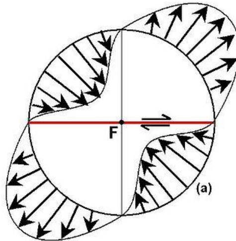
Schematic diagram showing the direction of initial movement of particles around the focus (F) of an earthquake on a W-E dextral strike-slip fault, viewed from above (a) and the equivalent zones of compressional (C) and tensional (T) sense first motion in the seismic waves radiating outward (b).
