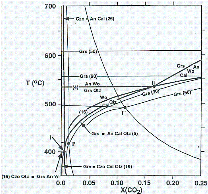
Figure 9. Water-rich [0.0 to 0.25 X(CO 2 )] portion of an isobaric (P T = P f = 100 MPa) T-X(CO 2 ) diagram illustrating the effects of solid solution (dilution of Grs with Adr, of Czo with Pi) on the phase equilibria of Figure 7. Shifts in location of equilibria calculated with methods described in the Thermodynamics section.
