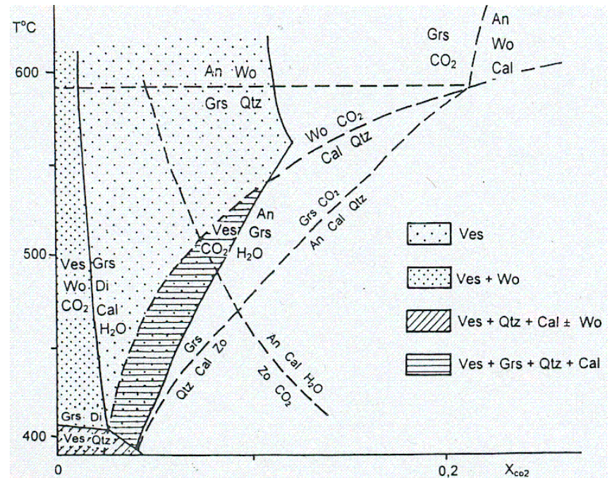
Obr. 1. Schematický T - X CO 2 diagram vybraných reakcí v systému CMAS-H 2 O-CO 2 při P fluid = P celk. = 200 MPa (upraveno podle Valleyho et al. 1985 a Labotka et al. 1988). Fig. 1. Schematic T - X CO 2 diagram showing selected reactions in the system CMAS-H 2 O-CO 2 at P fluid = P total = 200 MPa (modified from Valley et al. 1985 and Labotka et al. 1988).
