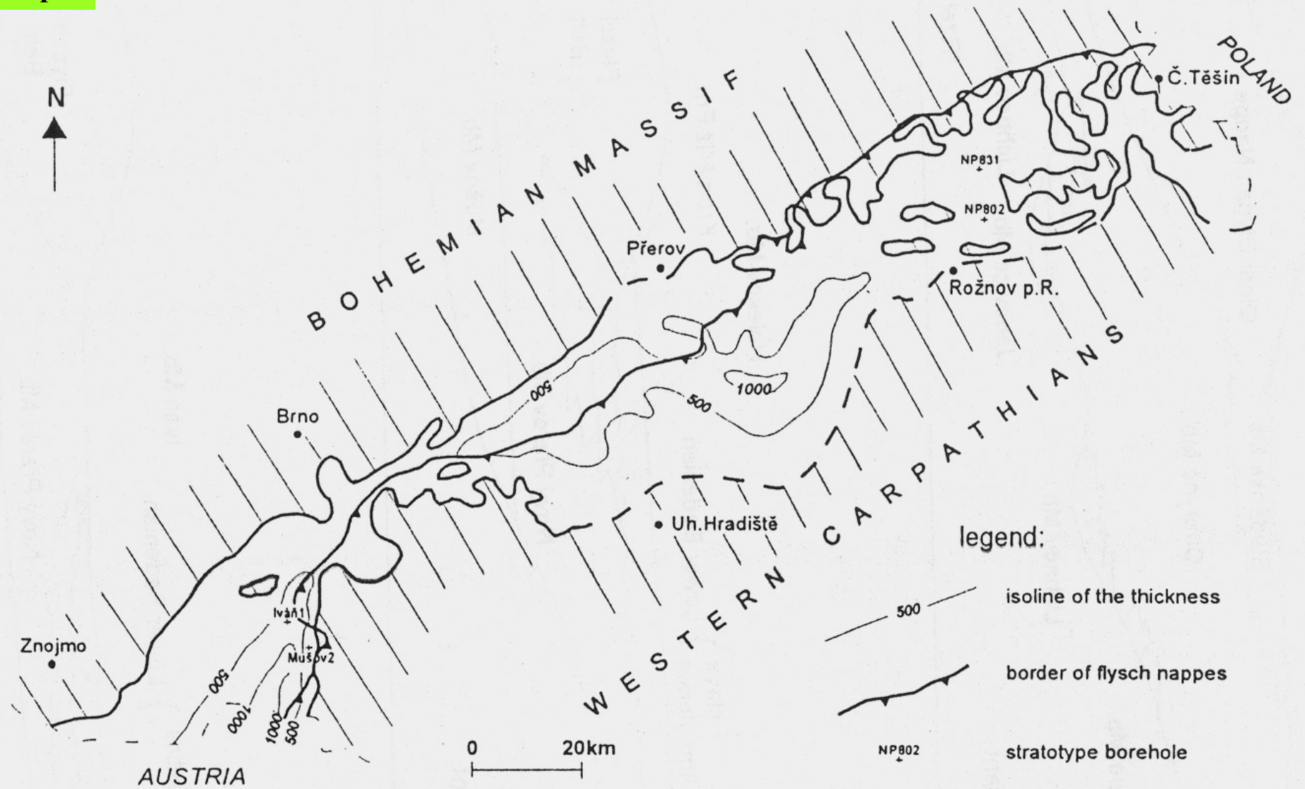
Figure 1: Thickness map of the Karpatian deposits of the Carpathian Foredeep (Moravia). (Adámek et al. 2003)
