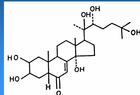
20-Hydroxyecdysone
