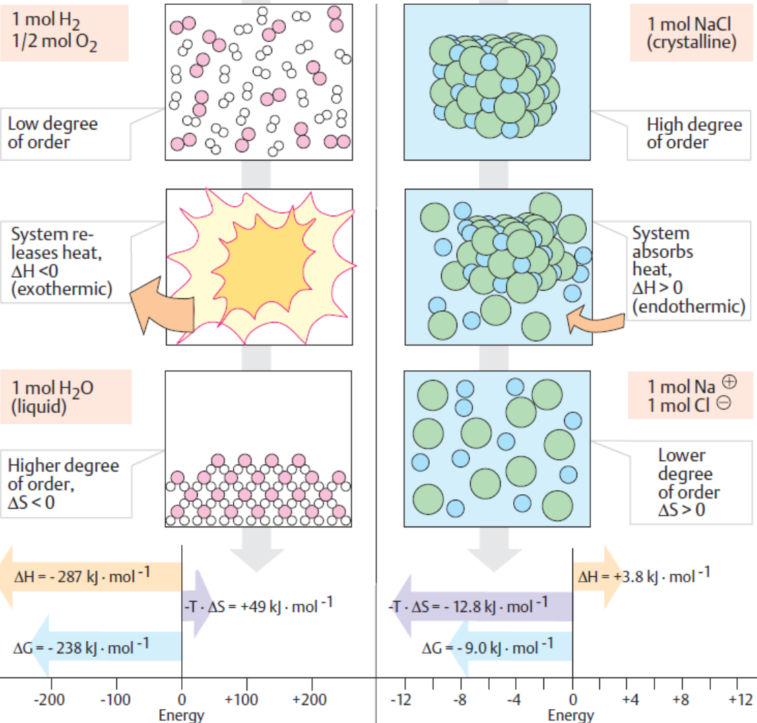
1. "Knall-gas" reaction
