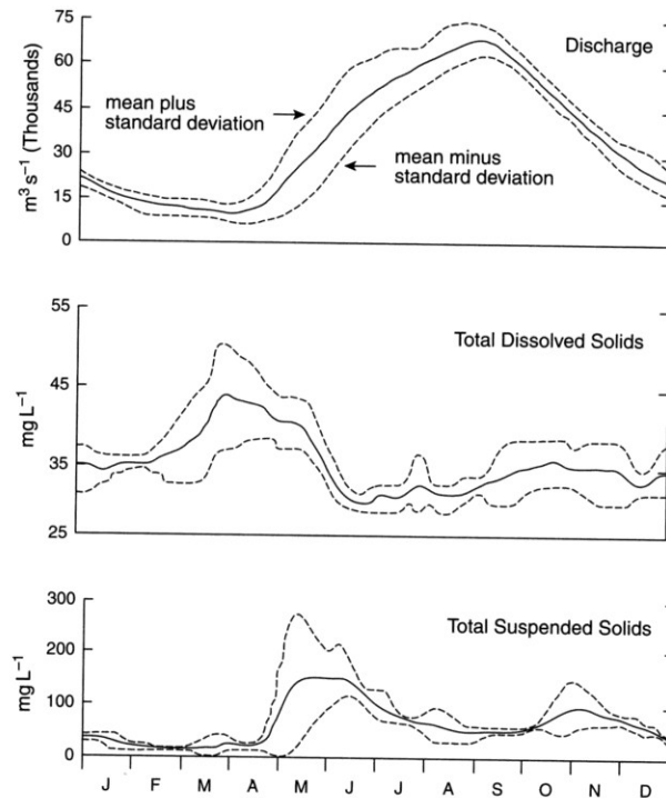
FIGURE 12 Illustration of seasonal changes in concentrations of dissolved and suspended solids in a large tropical river (the Orinoco). Standard deviations indicate interannual variation for a given time of the year. Redrawn from Lewis and Saunders (1989), with permission from Springer-Verlag.
