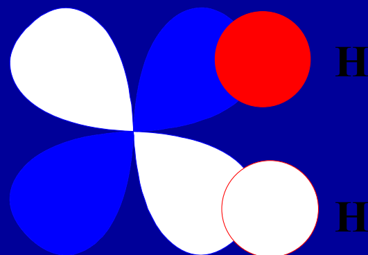
d\pi-\sigma^* H_2, R_3P, \text{alkany}
