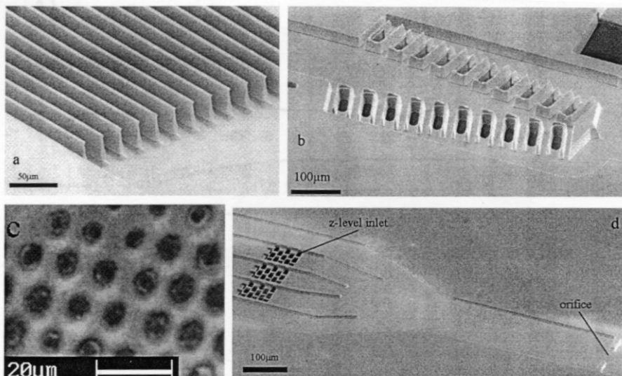
Fig. 6. Scanning electron microphotographs of some microfabricated devices. a) Immobilization reactor with 5 \mu\text{m} wide lamellas in a 50 \mu\text{m} deep channel. b) A mixer structure in a 50 \mu\text{m} deep channel. c) Inlet filter: Silicon membrane (15 \mu\text{m} ) with laser micromachined pores. d) Coulter sizer setup with 5 planar inlets and a z-level inlet.
