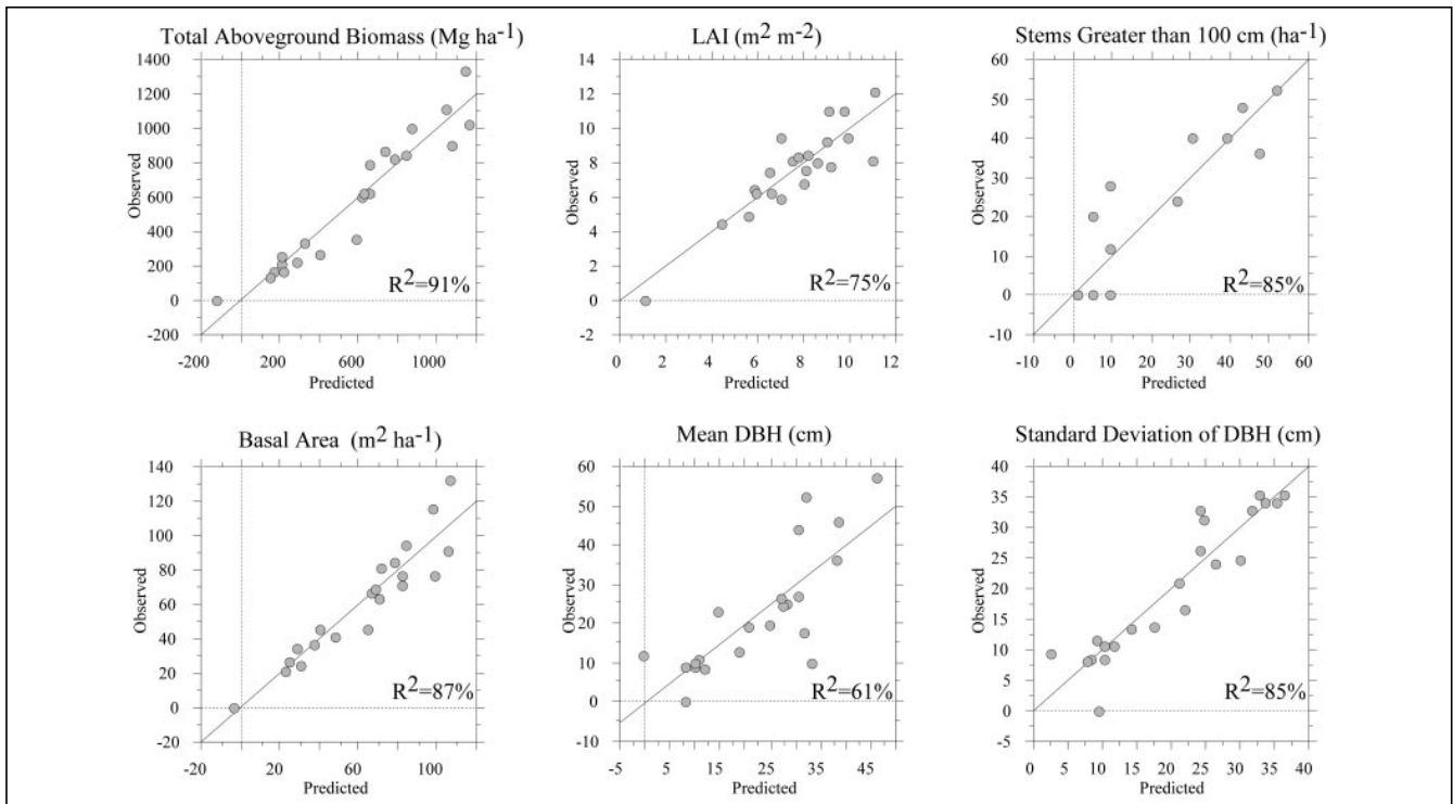
Figure 9. Scatterplots of predicted and observed stand attributes from 22 plots at the H. J. Andrews Experimental Forest. Figure adapted from Lefsky et al. (1999b), with permission from Elsevier Science.
