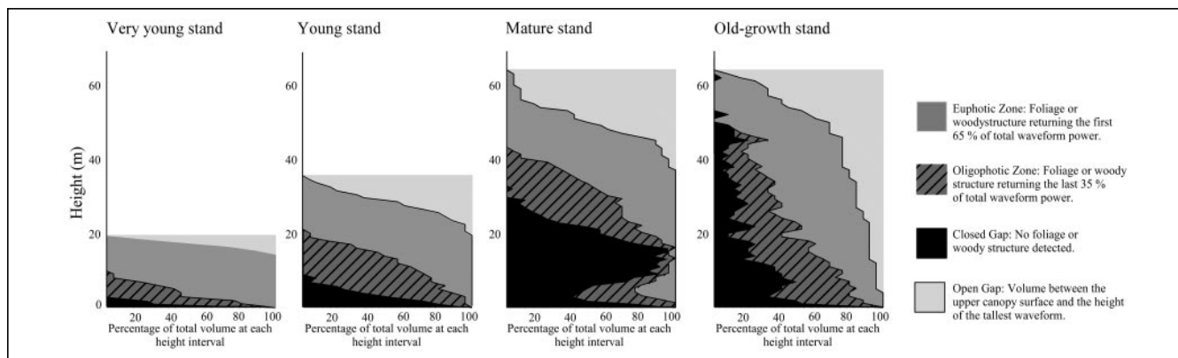
Figure 8. Canopy volume profile diagrams for representative young, mature, and old-growth Douglas-fir and western hemlock forest plots. These diagrams indicate, for each 1-meter vertical interval, the percentage of each plot's 25 waveforms that belong to each of the four canopy structure classes. Young stands are characterized by short stature, a uniform upper canopy surface, and an absence of empty space within the canopy. Mature stands are taller, characterized by a uniform upper canopy surface but with a large volume of empty space within the canopy. Old-growth stands are distinguished from mature stands by their uneven canopy surface and the broad vertical distribution of each of the four canopy structure classes. Whereas stands from earlier stages in stand development have canopy structure classes in distinct vertical layers, in the old-growth stands each canopy structure class occurs throughout the height range of the stands. This trait has been cited as a key physical feature distinguishing old-growth forests from the simpler canopies of young and mature stands (Spies and Franklin 1991). Figure adapted from Lefsky et al. (1999b), with permission from Elsevier Science.
