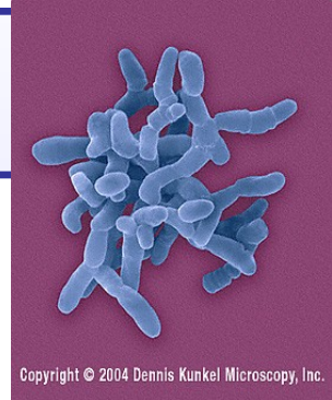
Mycobacterium paratuberculosis
