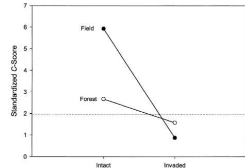
Figure 2 Effects of S. invicta on community structure. The standardized C -score measures the extent to which species occur less frequently than expected by chance. The larger the standardized C -score, the less co-occurrence compared with a randomly assembled community. The dotted line indicates 1.96 standard deviations, the approximate level of statistical significance ( P < 0.05 ). ○, Forest ant assemblages; ●, open-field ant assemblages. In the presence of S. invicta , ant community structure converges to a random pattern.
