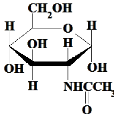
N-ACETYLGLUKOSAMIN
