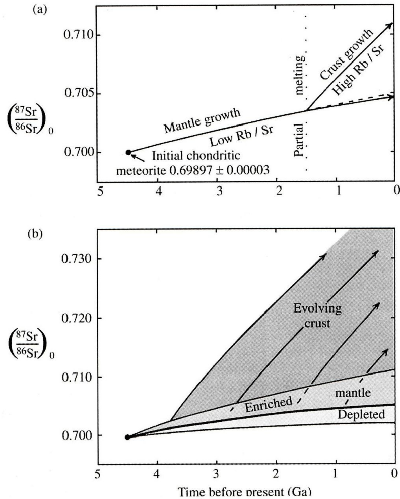
2.26 Schematic strontium isotope evolution diagrams for the Earth. Filled circle represents an assumed parental chondritic meteorite whose initial (^{87}\text{Sr}/^{86}\text{Sr})_0 ratio at 4.5 Ga, when the Earth accreted from primordial material, was 0.69897 \pm 0.00003 . Note that growth lines are slightly curved because the amount of ^{87}\text{Rb} decaying to ^{87}\text{Sr} decreases through time. (a) Single-stage model with hypothetical partial melting event at 1.5 Ga. Thereafter, mantle growth is at a slightly lower rate because of extracted Rb from a depleted mantle. (b) Multistage model in which the mantle has been partially melted many times throughout its history to create a growing, evolving crust. Metasomatic processes create an incompatible-element- enriched mantle (Section 11.2.2); other parts of mantle are relatively depleted through partial melting processes.
